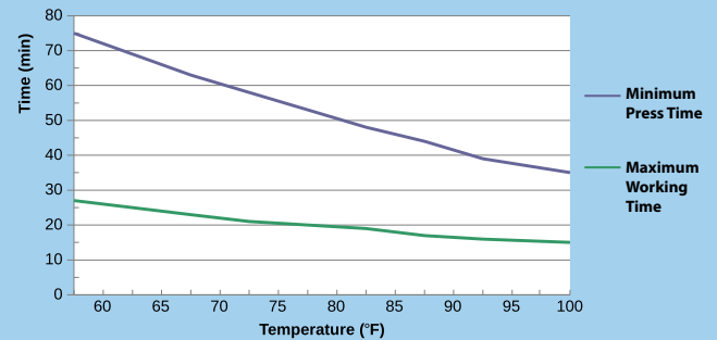
Estimated Cure Time for OnePart 20
